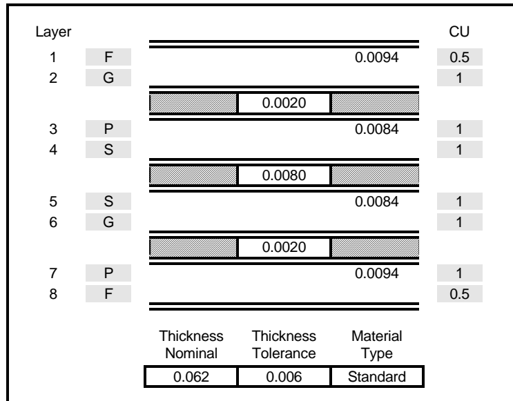
Eight Layers (Buried Capacitance)
